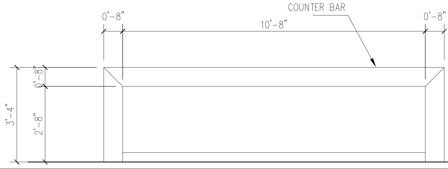
INTERIOR VIEW C-C BAR AREA SCALE : 1/2" = 1'-0"
