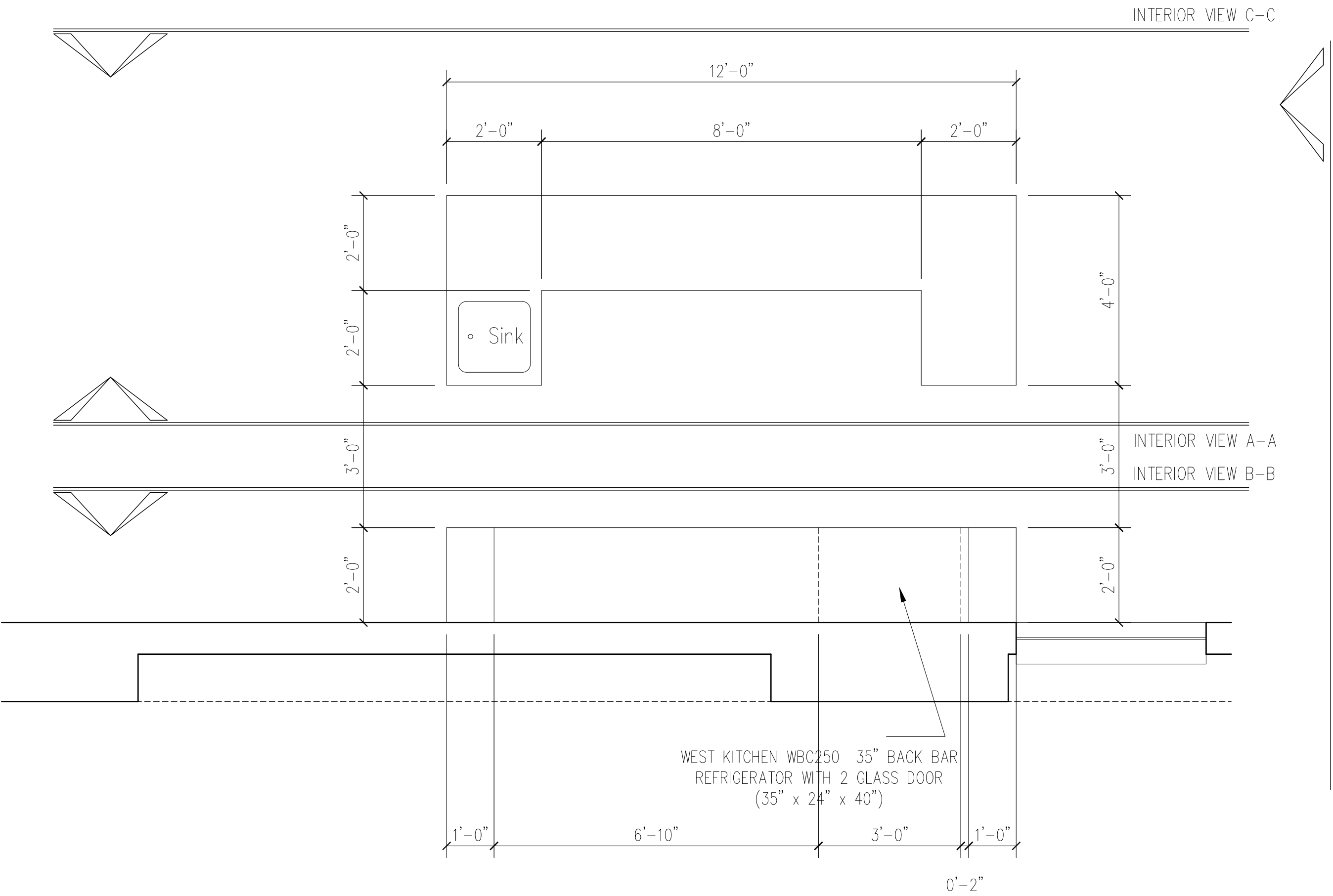
NEW FLOOR PLAN BAR AREA SCALE : 1/2" = 1'-0"
