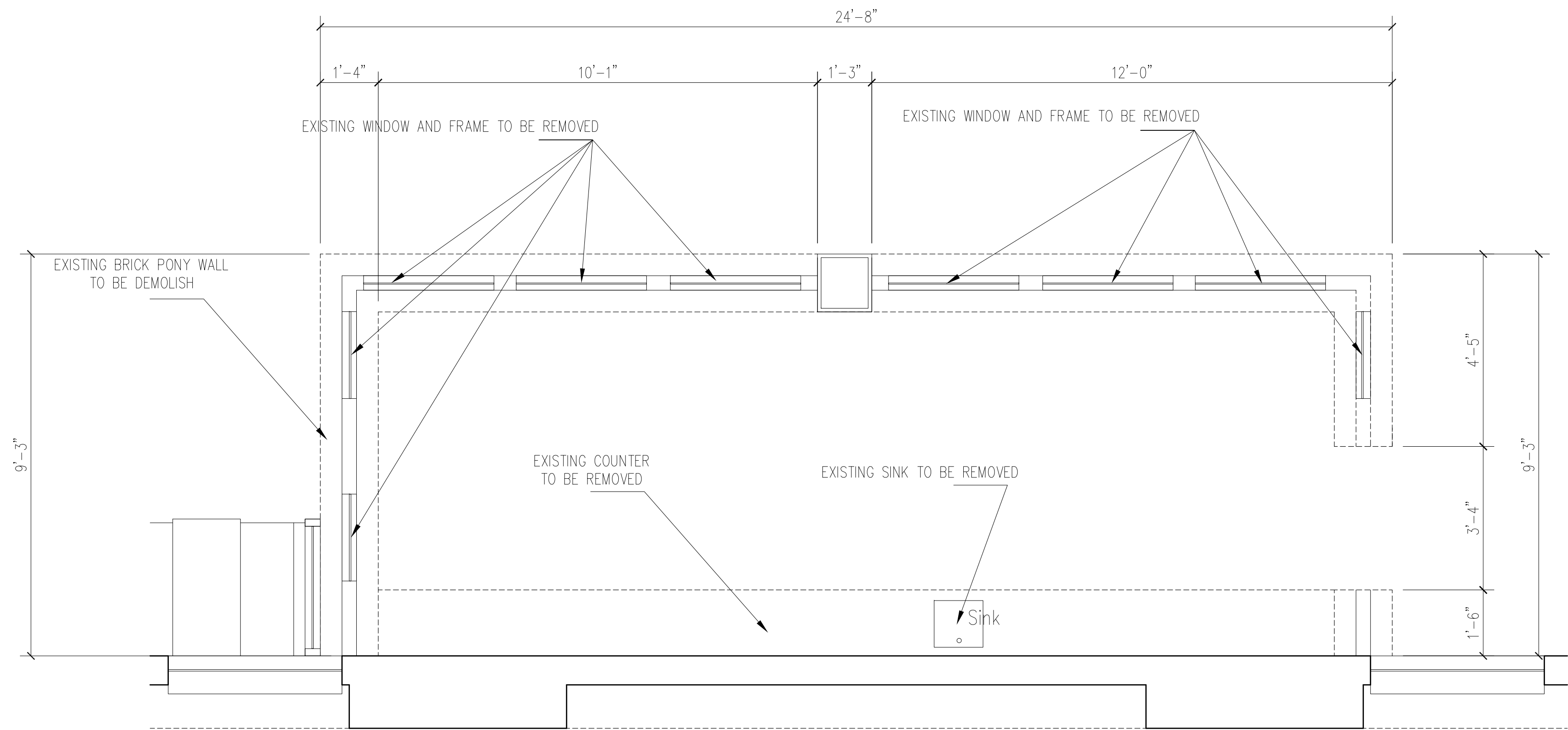
EXISTING FLOOR PLAN BAR AREA SCALE : 1/2" = 1'-0"
