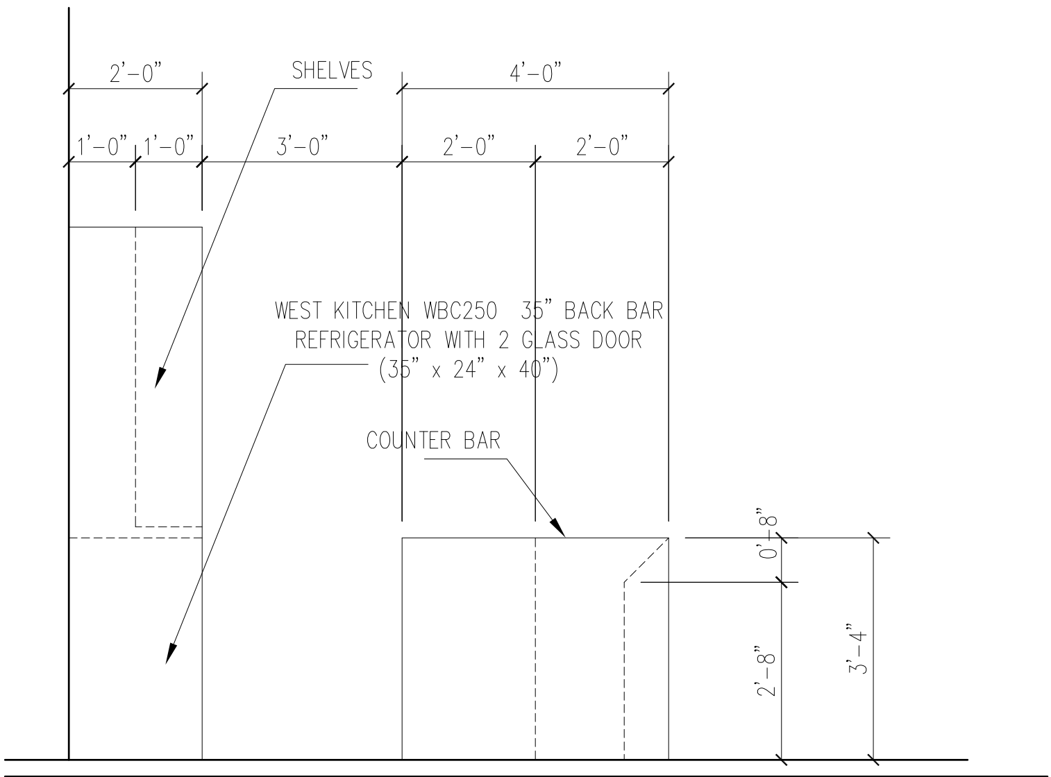
INTERIOR VIEW D-D BAR AREA SCALE : 1/2" = 1'-0"
