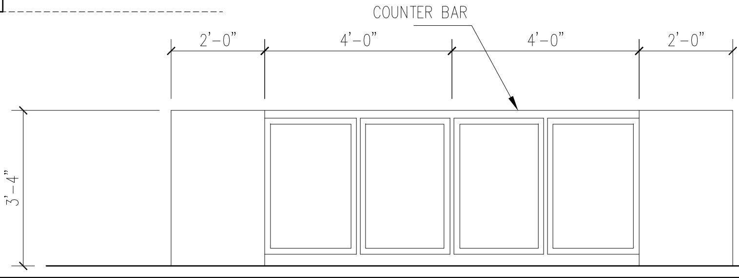
INTERIOR VIEW A-A BAR AREA SCALE : 1/2" = 1'-0"
